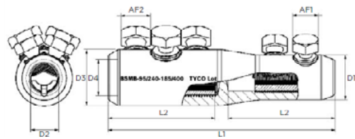
Reduction Connector
