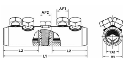
Split Connector
